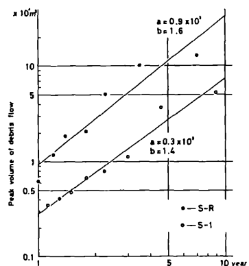
Fig.5 Peak Volume of Debris Flows and Frequency
