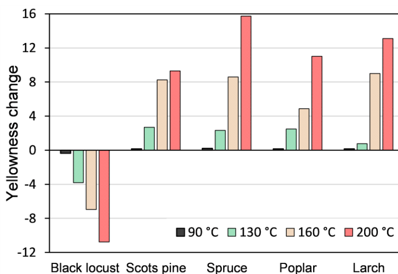
Figure 7. Yellowness change of different wood species generated by 6-hour dry thermal treatment at different temperatures
