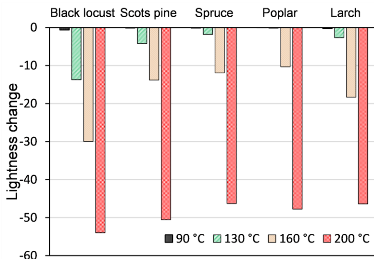
Figure 5. Lightness change of different wood species generated by 6-hour dry thermal treatment at different temperatures
